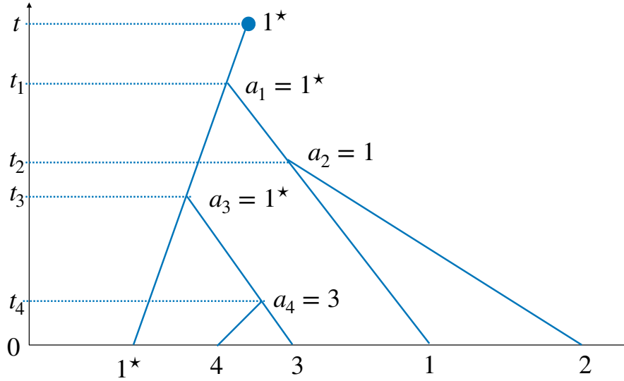
Figure 3.1: The history of the particle 1^* can be encoded in a tree a , say of size n , whose root is indexed by 1^* . The pseudotrajectory is then prescribed by the collision parameters (t_i, v_i, \omega_i)_{1 \leq i \leq n} .
