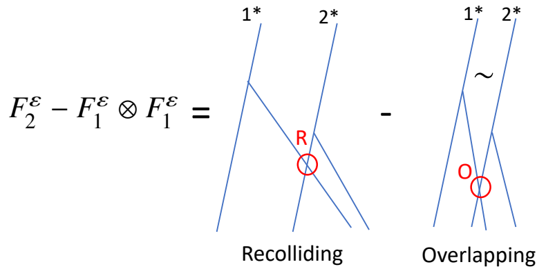
Figure 3.4: The second-order cumulant corresponds to the occurrence of at least one recollision between trees or an overlap.
