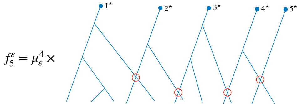
Figure 3.5: The cumulant of order k corresponds to trees with roots in 1^*, \dots, k^* that are completely connected by external collisions or overlaps.
