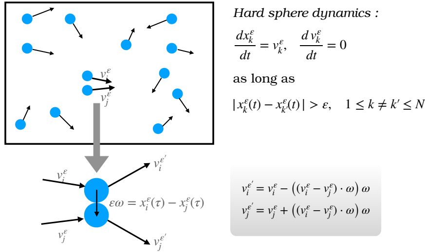
Figure 1.1: At time t , the system of hard spheres is described by the positions (x_k^\varepsilon(t))_{k \leq N} and the velocities (v_k^\varepsilon(t))_{k \leq N} of the N particles' centers of gravity. The spheres move in a straight line and when two of them touch, they are scattered according to elastic reflection laws.
