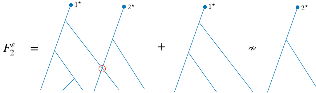
Figure 3.2: F_2^\epsilon trees are classified into two categories: those involving an (external) collision between the 1^* and 2^* trees, and others for which the particles in the 1^* tree are always at least \epsilon away from those in the 2^* tree (which we denote by \approx ).
