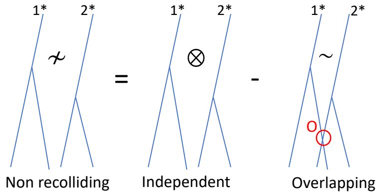
Figure 3.3: Decomposition of the dynamical exclusion condition.
